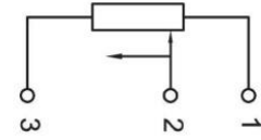
Potentiometer Connection (Voltage Divider)
